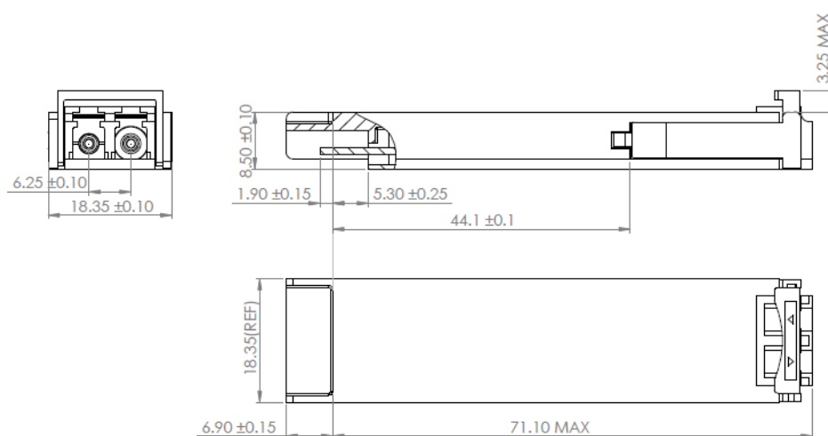
10G-X-SR(dimensions are in mm)
