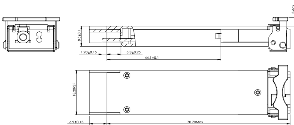
10G-BX3327-ER(dimensions are in mm)
