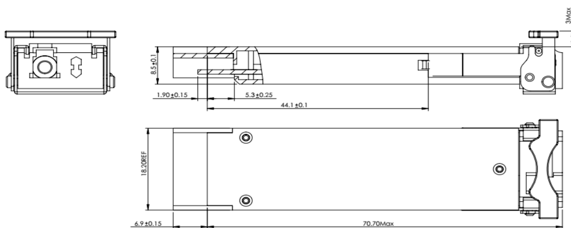
10G-BX2733-LR(dimensions are in mm)
